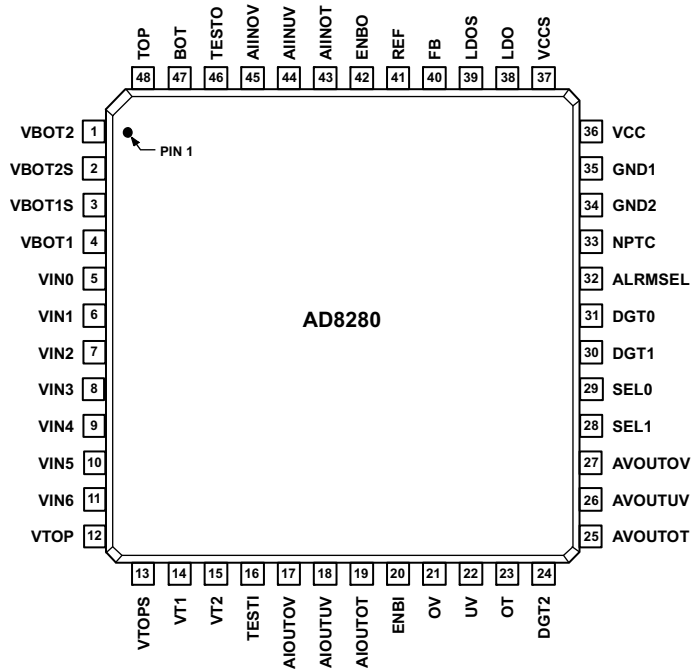
Figure 2. Pin Configuration
